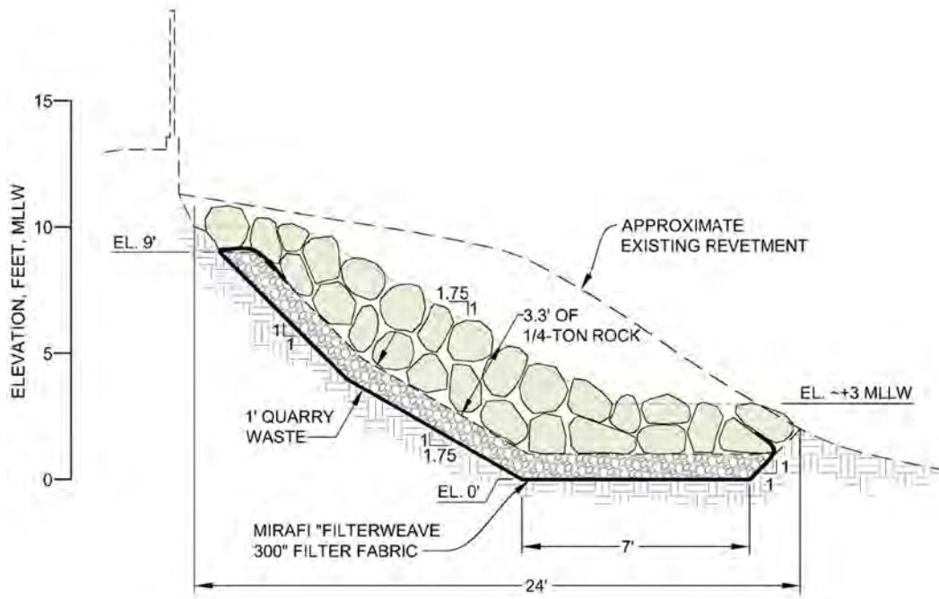
Figure 5. New Revetment Elevation View.
