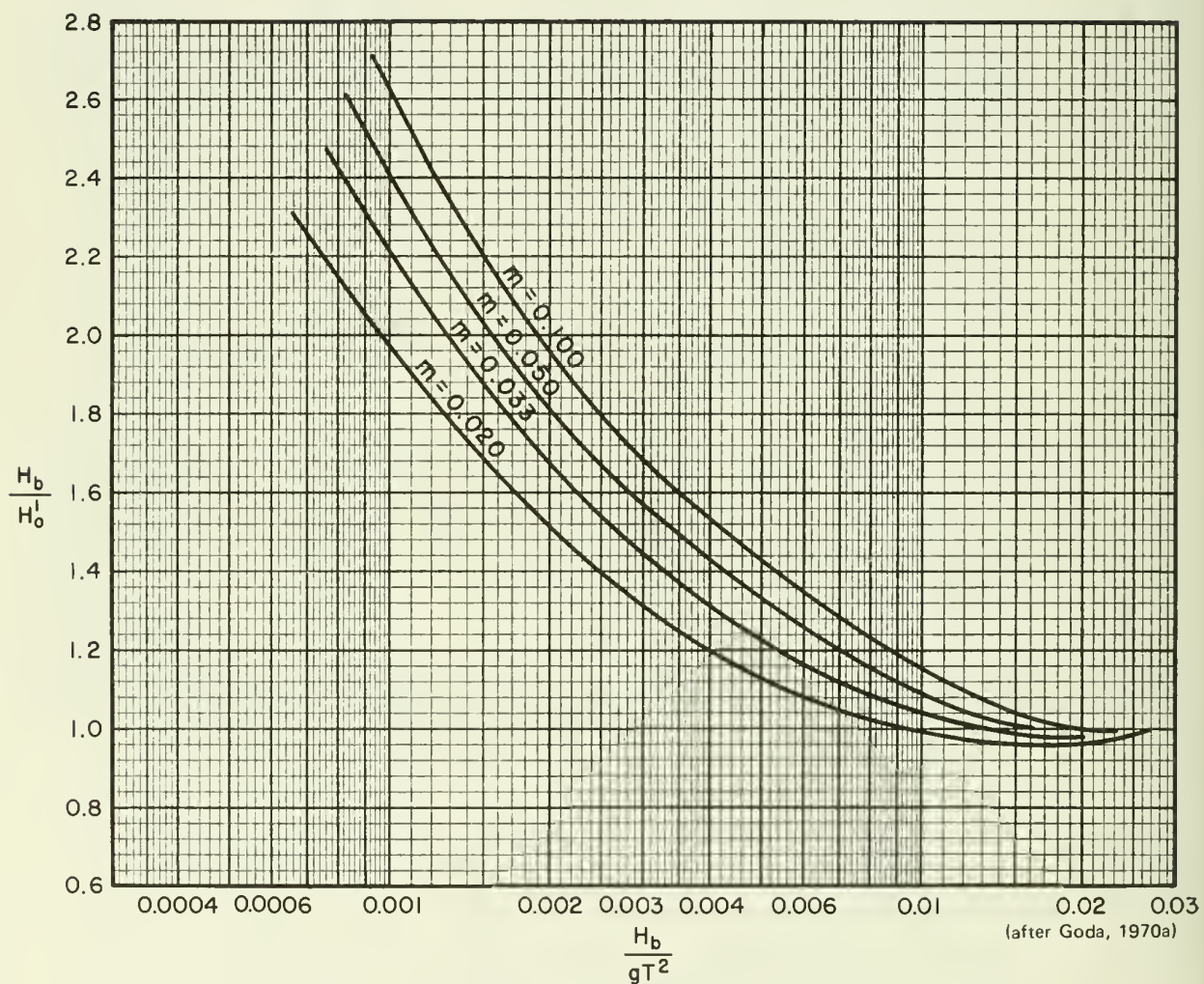
Figure 7-5. Breaker height index H_b/H_0 versus H_b/gT^2 .
