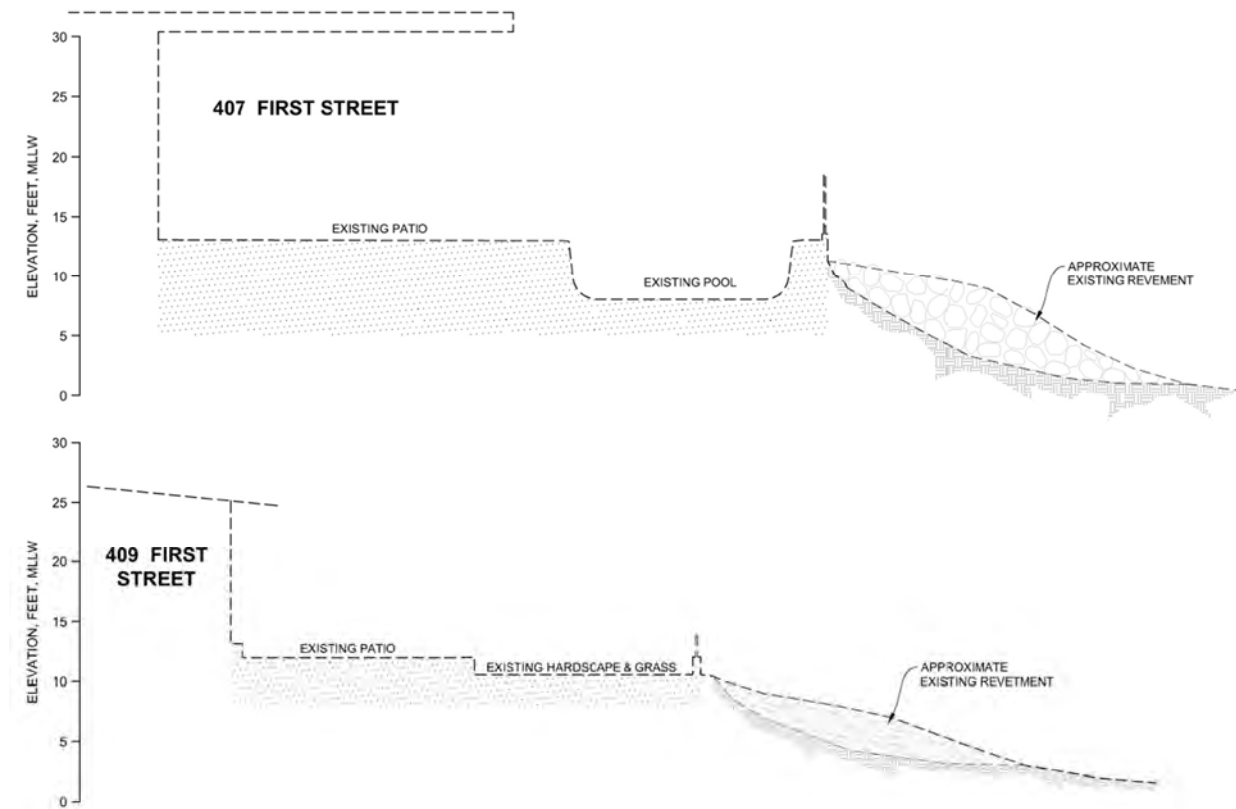
Figure 4. Existing Revetment Elevation Views.
