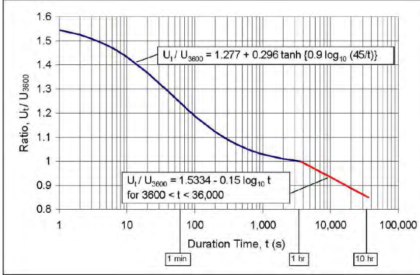
Figure 12. Coastal Engineering Manual Wind Duration Conversion.
