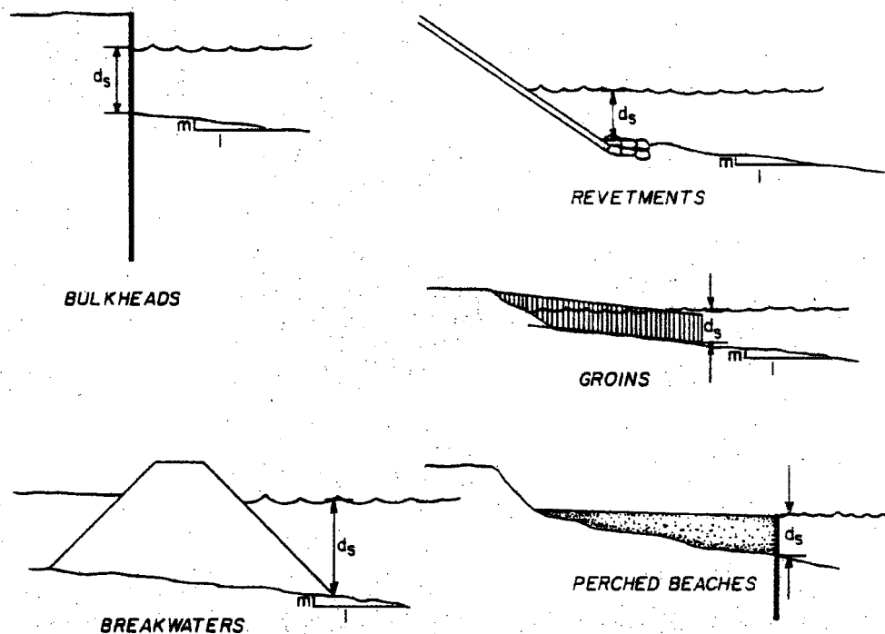
Figure 19 Depth at Structure for Various Devices
