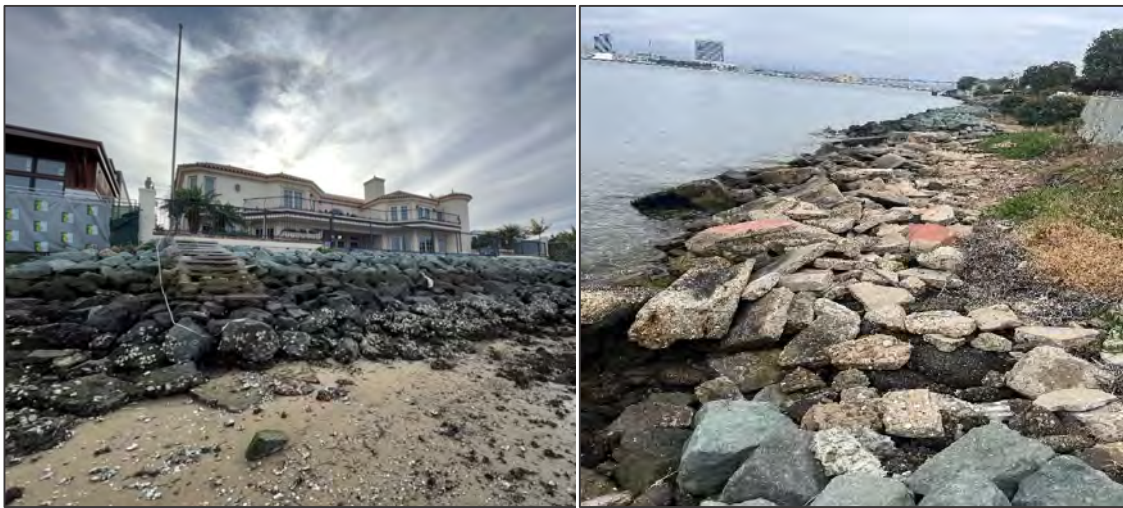
Figure 3. Existing Revetment Site Images.
