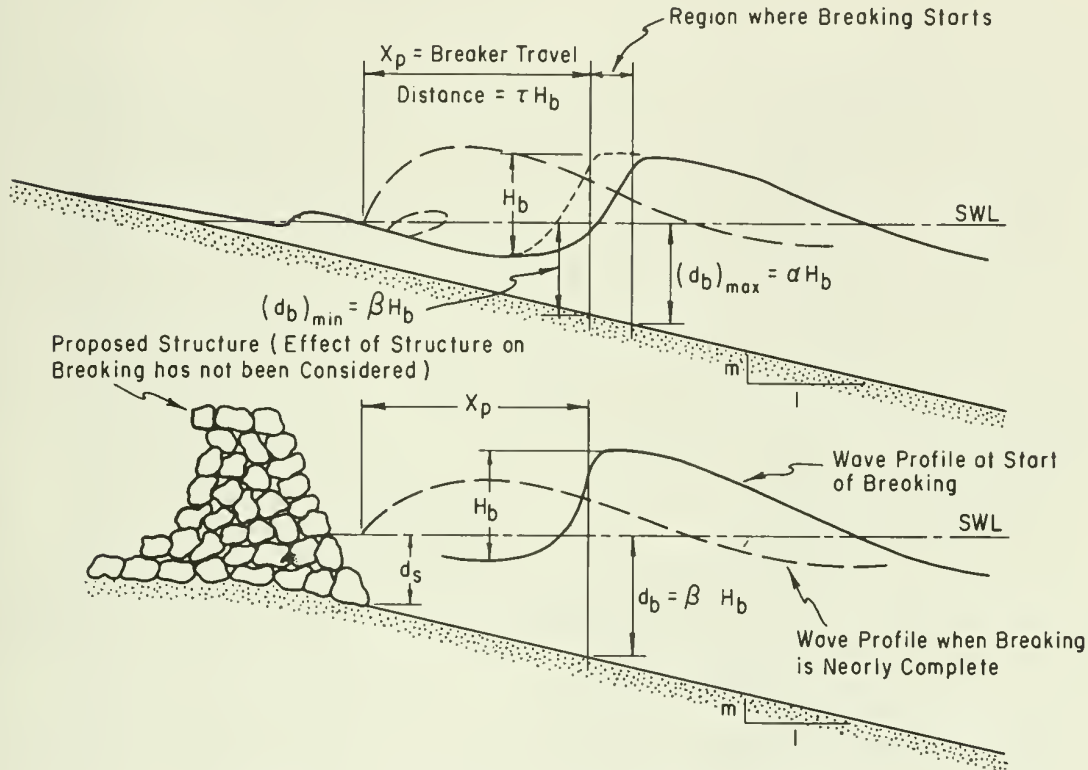
Figure 7-1. Definition of breaker geometry.
