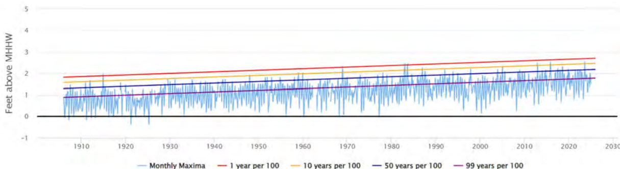
Figure 8. NOAA Extreme Water Levels for Station 9410170 San Diego.
