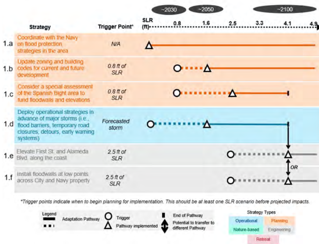
Figure 17. Project Vicinity Adaptation Pathway.
