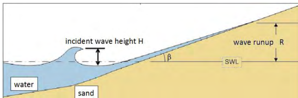
Figure 14. Wave Runup Illustration.
