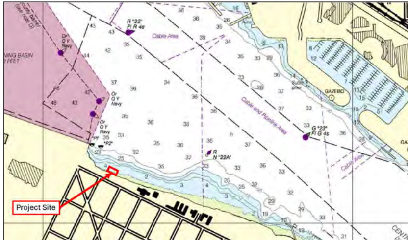
Figure 11. Project Site Vicinity Bathymetry.
