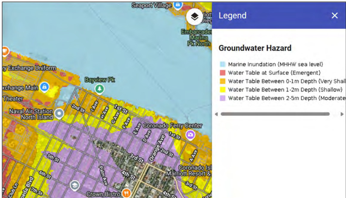
Figure 15. CoSMoS Groundwater Rise Model with 4.9 Feet of Sea Level Rise.
