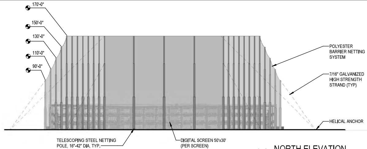
02 NORTH ELEVATION SCALE: 1/64" = 1'-0"
